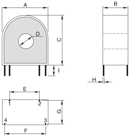
DIMENSIONS IN:mm
